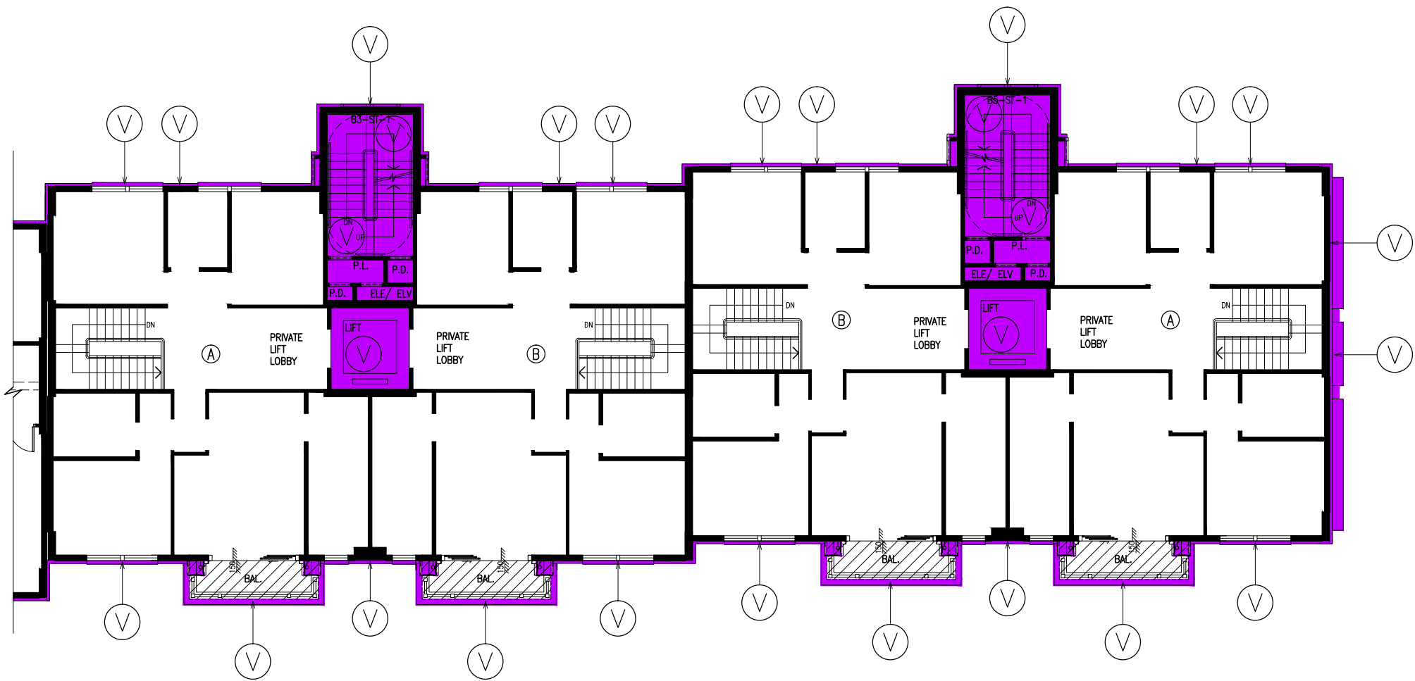
BLOCK 3 2ND FLOOR PLAN
