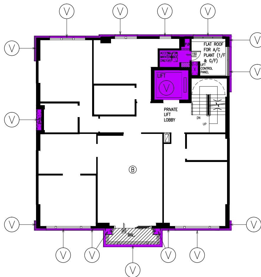
BLOCK 12 3RD FLOOR PLAN
