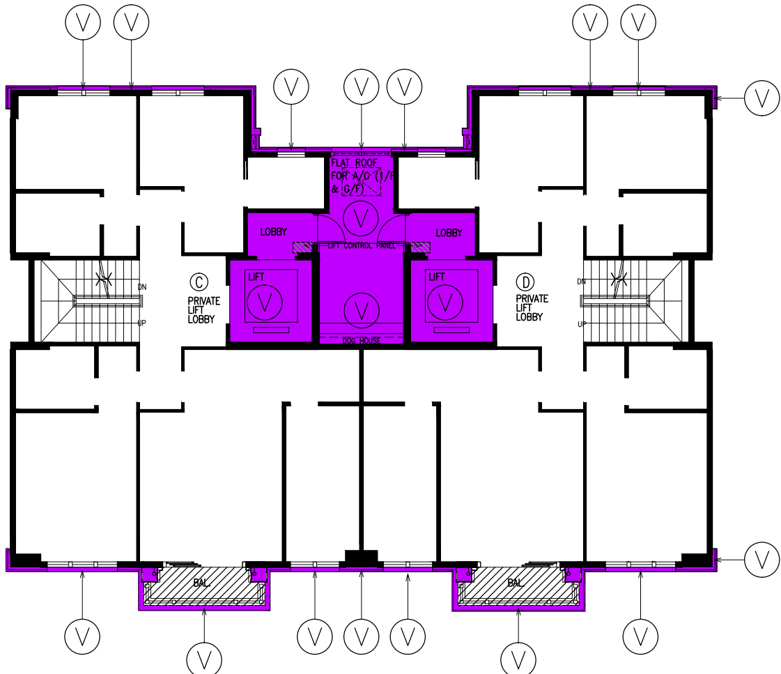
BLOCK 10 3RD FLOOR PLAN
