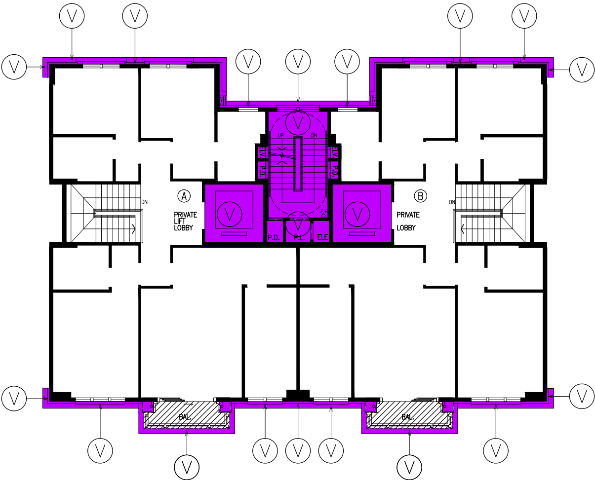
BLOCK 10 1ST FLOOR PLAN
