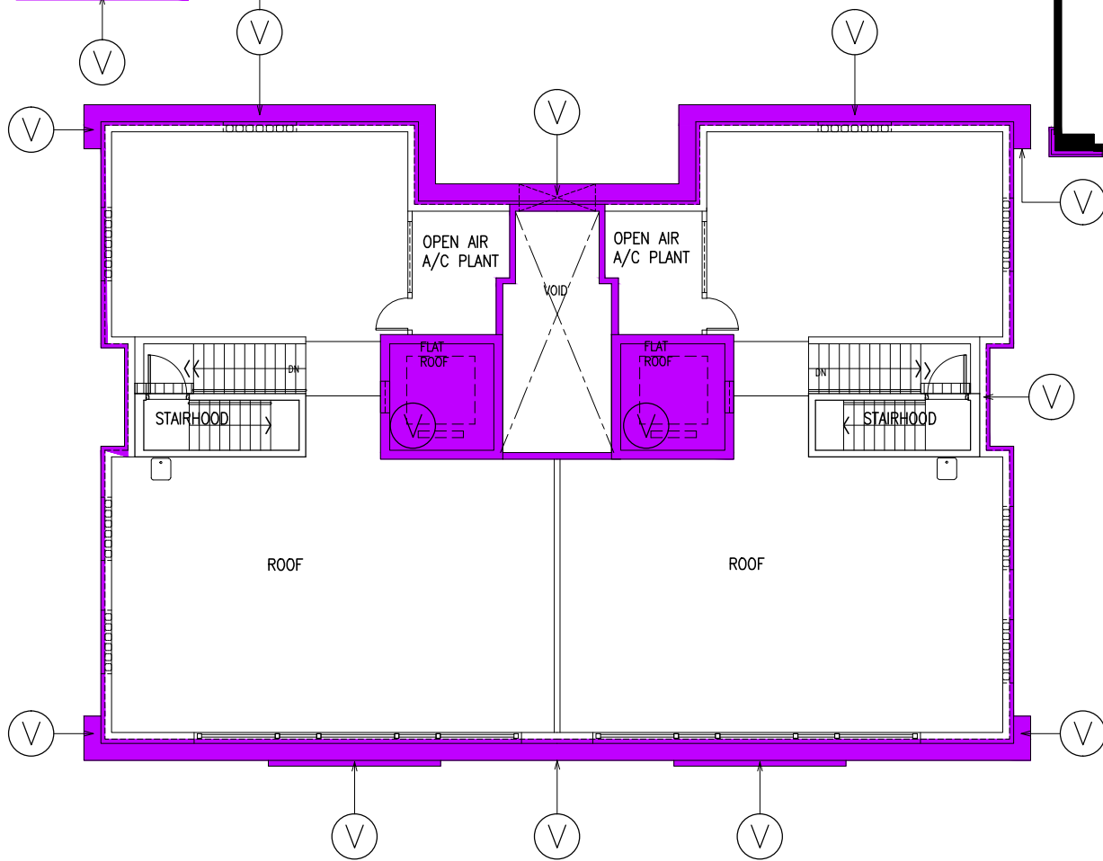
BLOCK 11 ROOF PLAN
