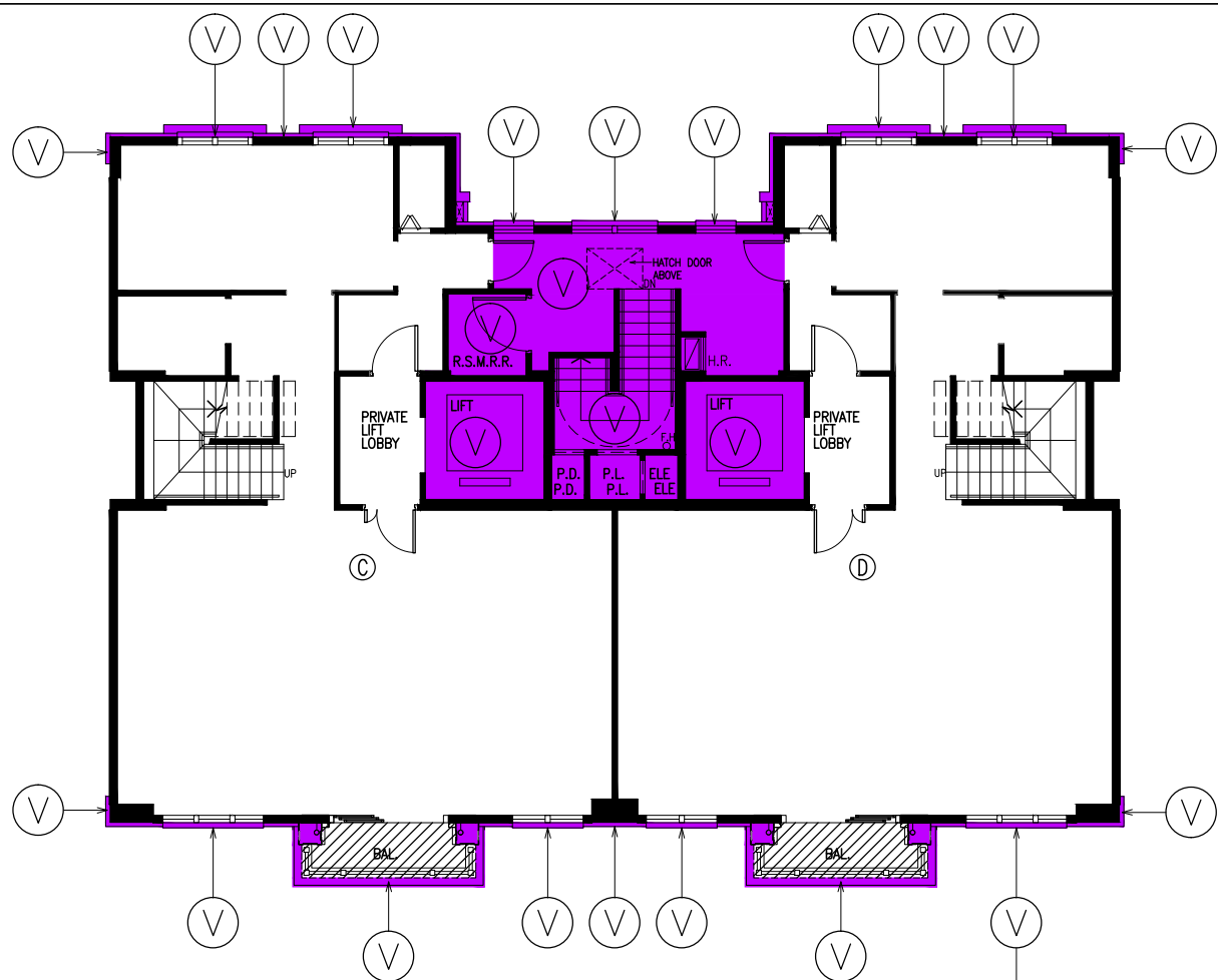
BLOCK 11 2ND FLOOR PLAN
