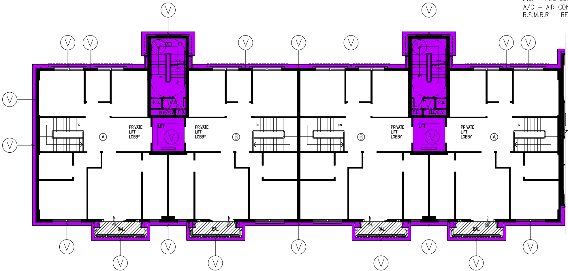
BLOCK 1 1ST FLOOR PLAN
