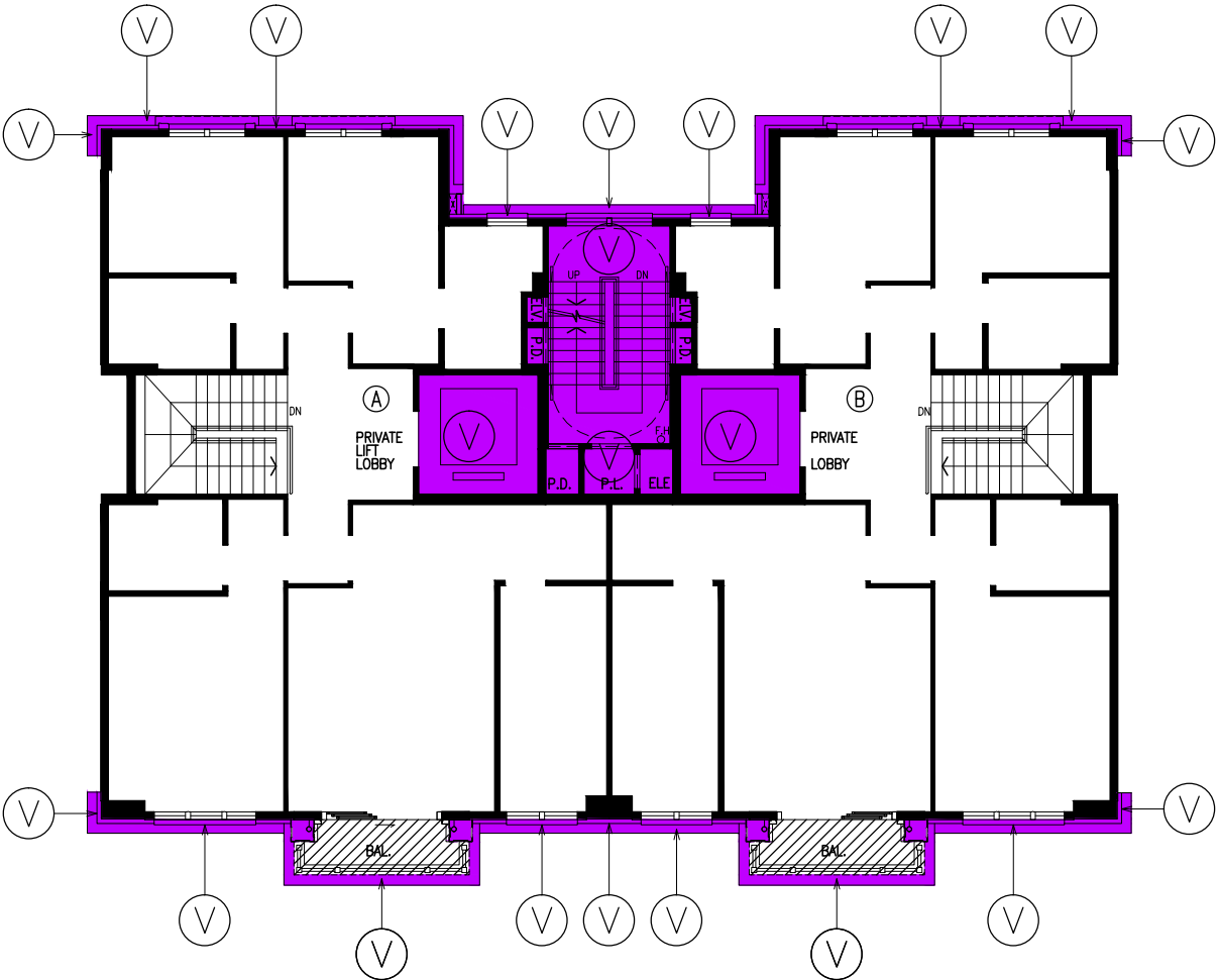
BLOCK 11 1ST FLOOR PLAN
