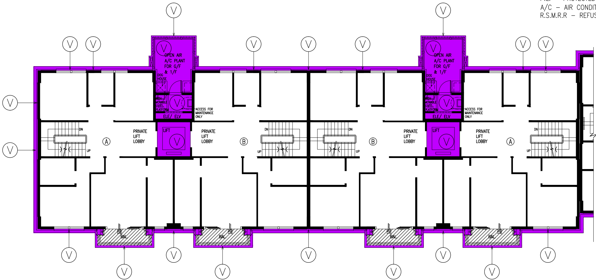
BLOCK 1 3RD FLOOR PLAN
