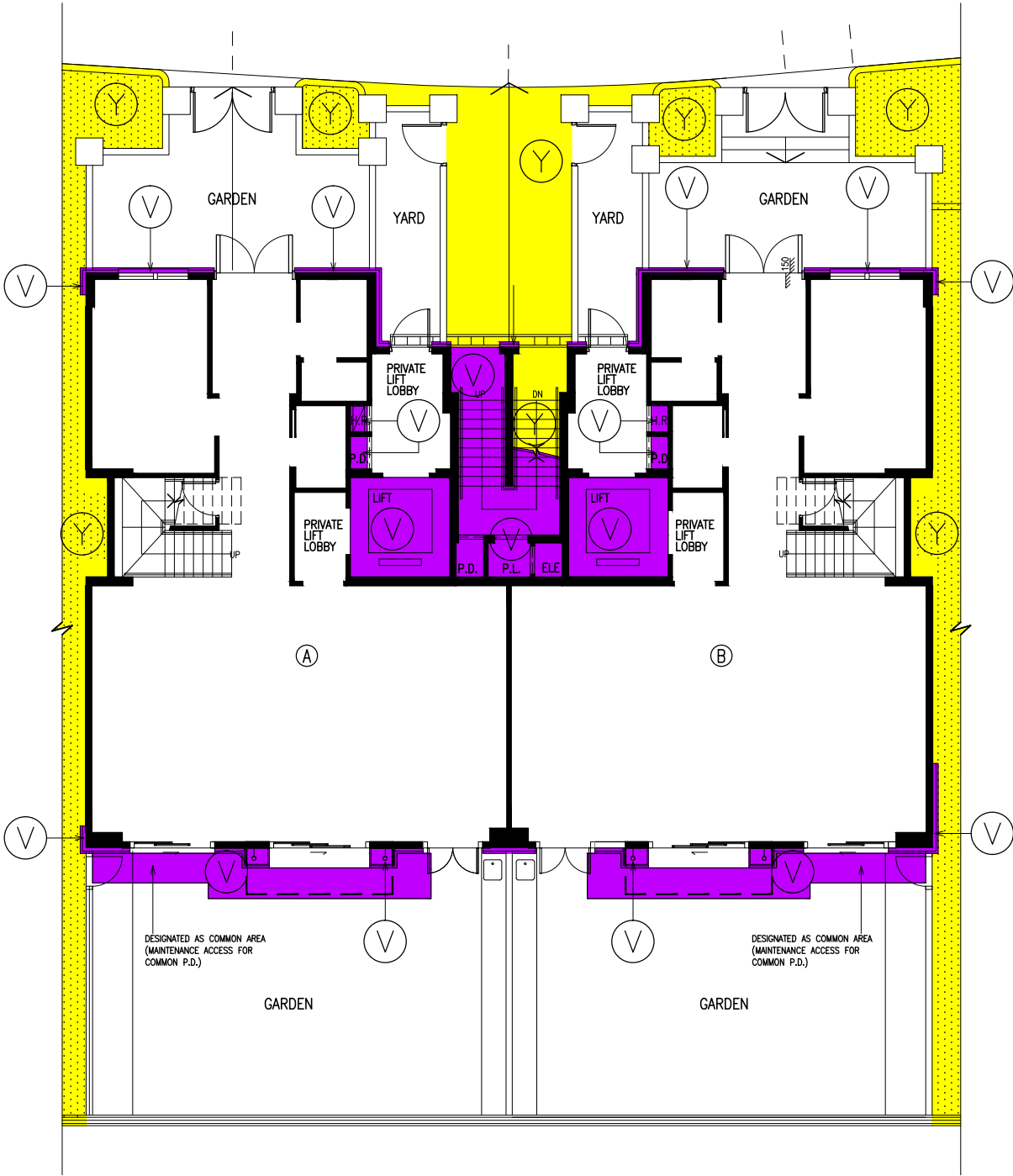
BLOCK 10 GROUND FLOOR PLAN
