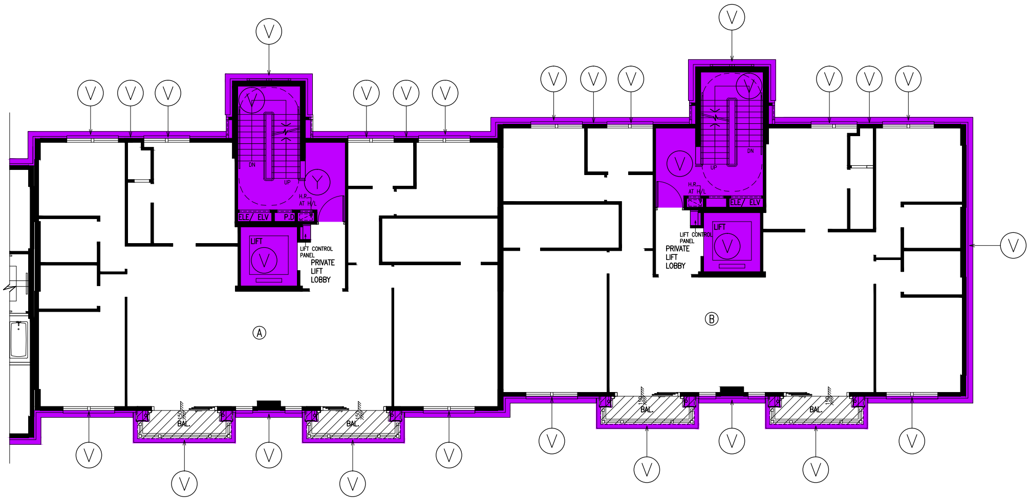
BLOCK 3 3RD FLOOR PLAN
